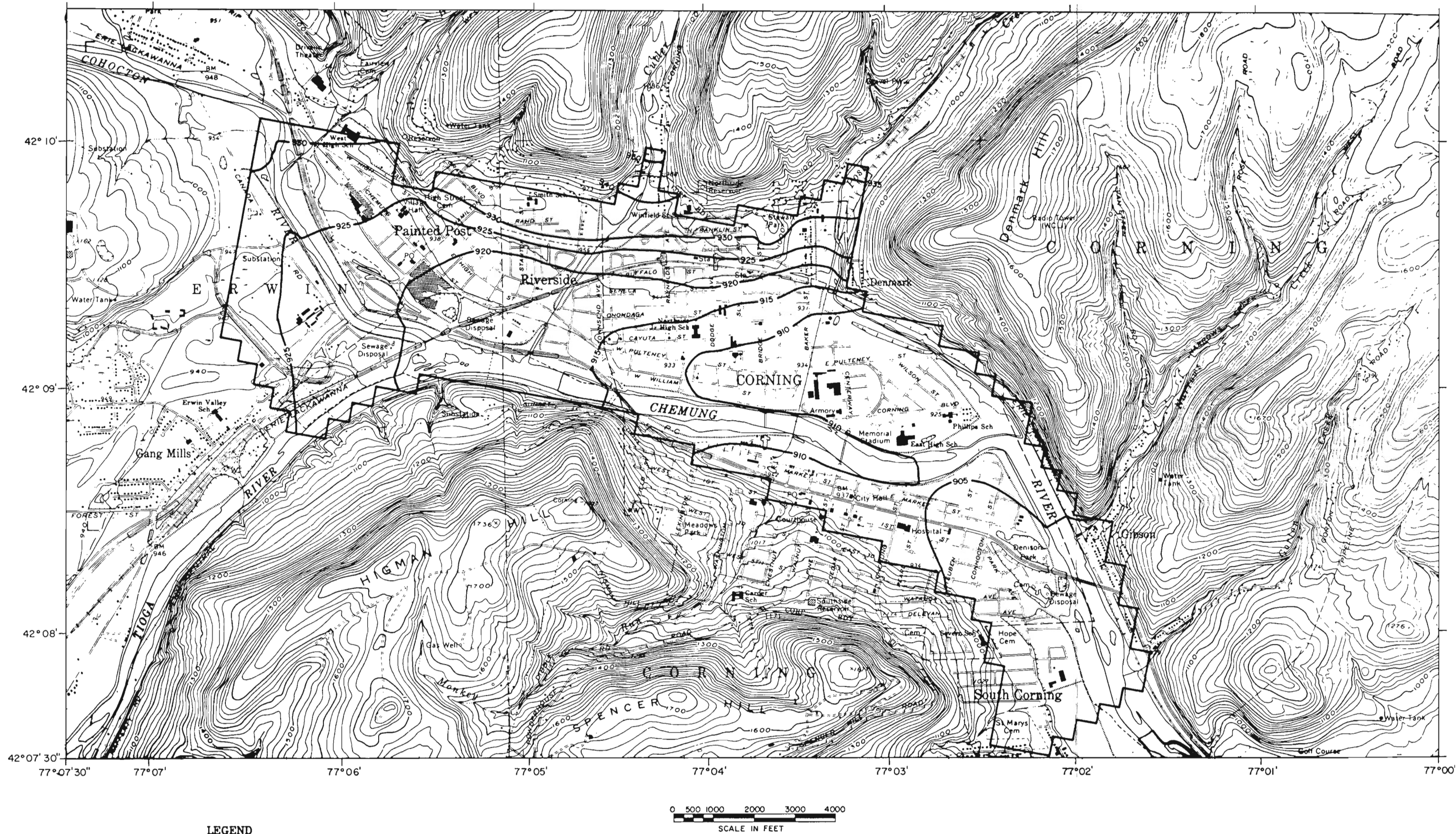
FIGURE 24. MAP SHOWING CALCULATED WATER LEVEL CONTOURS IN LAYER 1 FOR HYPOTHETICAL DROUGHT CONDITIONS.
